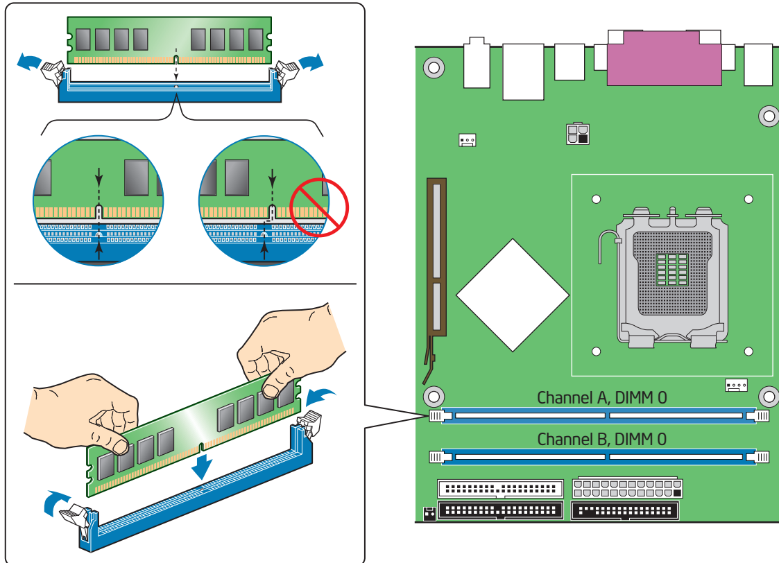
Figure 15. Installing a DIMM
